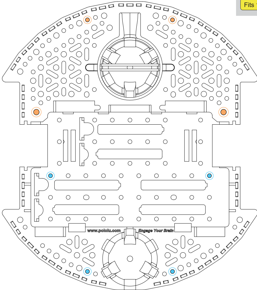
Romi Base Plate
