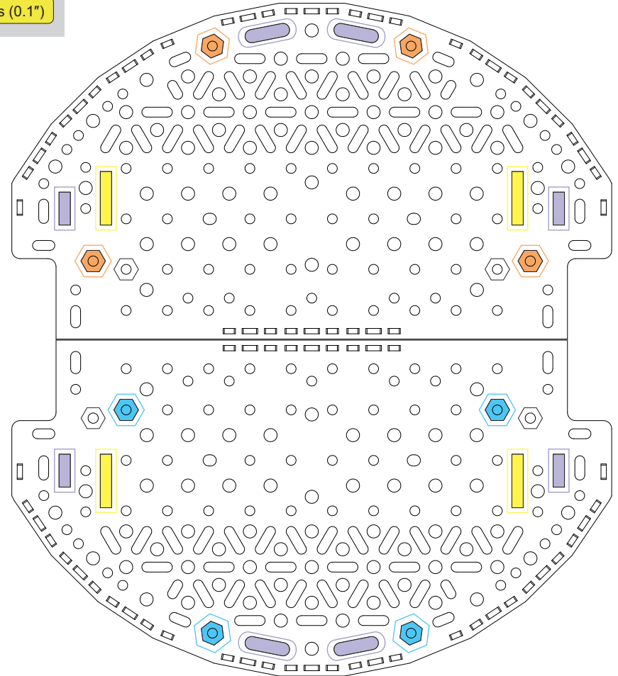
Romi Chassis Expansion Plates
